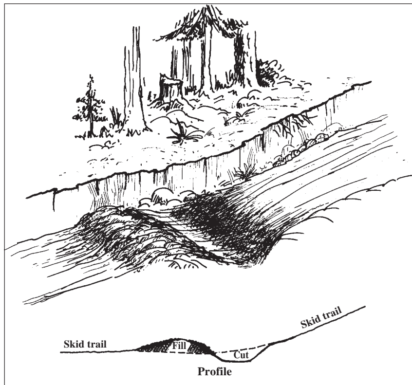
Figure 8.—Water bar construction.
