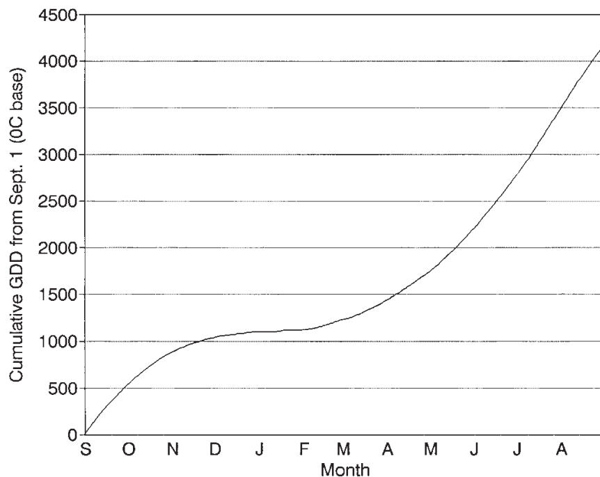
Figure 3. —Cumulative growing degree days (base 0° centigrade) for Pendleton, OR.
