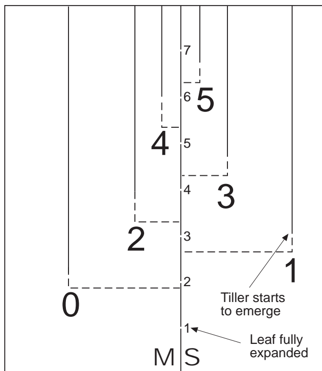
Figure 4. —Relationships of leaf and tiller production in winter wheat based on data for 'Stephens' wheat.
