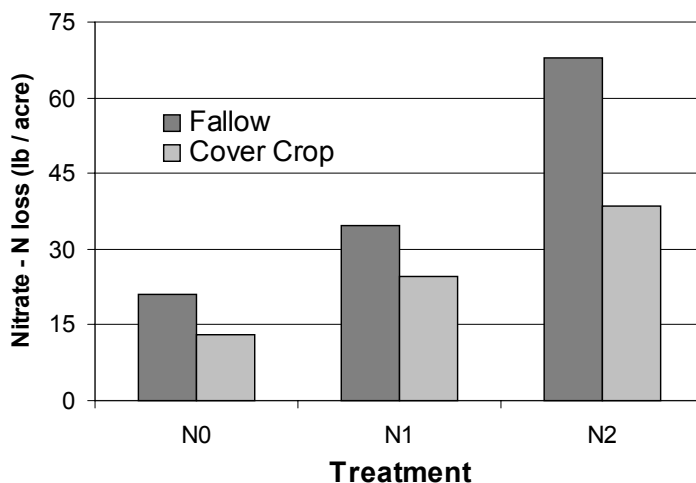
Figure 9. Average NO 3 - -N mass leaching rate for plots at the North Willamette Research and Extension Center during the first eight seasons using cereal rye cover crops. Crops were fertilized at three different rates, N0 received none; N1 half, and N2 the recommended agronomic rate to maximize crop yield.
