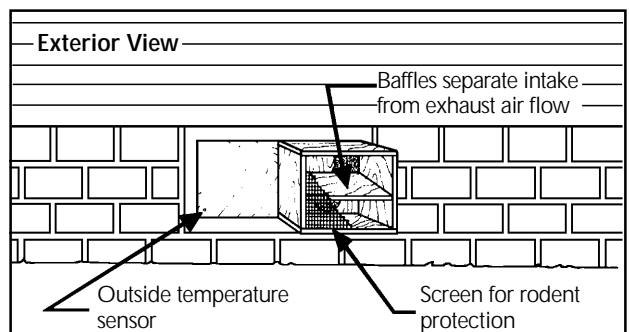
Figure 7. Basement storage ventilation system.
