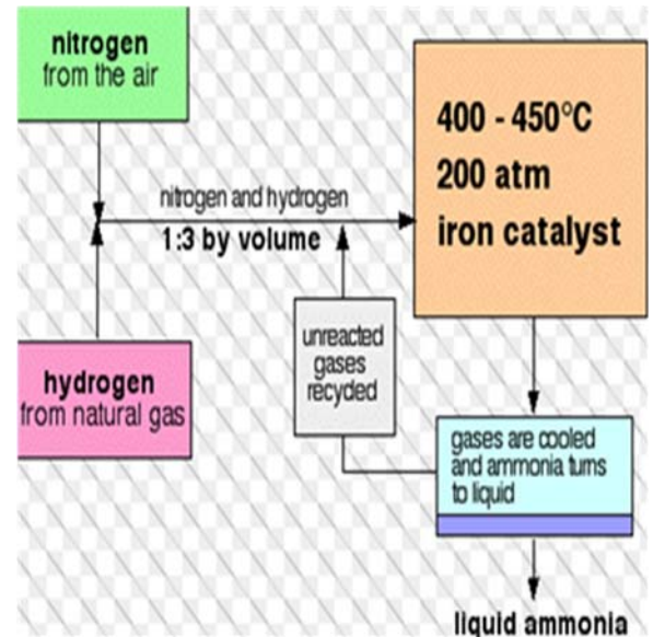
Figure 1 Schematic of Haber-Bosch.
