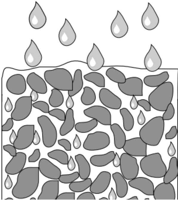
Figure 3. Soil with good structure has stable pore spaces that allow water penetration, root growth, earthworm movement, and air storage.
