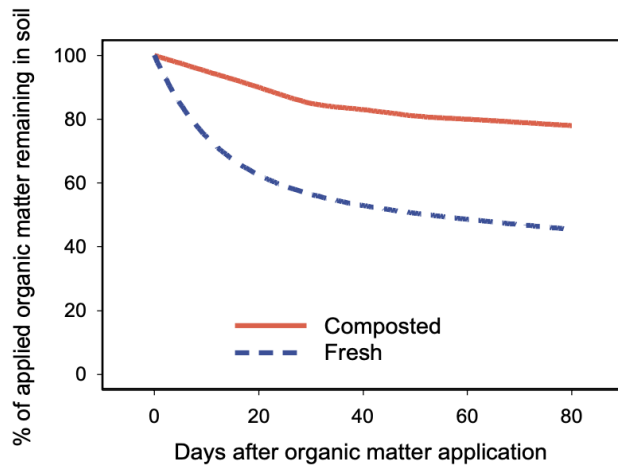
Figure 4. Fresh organic materials decompose more rapidly than composted organic materials. About half of fresh organic matter is lost from the soil as carbon dioxide gas during the first 60 days after soil incorporation. Composted materials increase soil organic matter for a longer time. About half of the composted organic matter is lost in the first 1 to 2 years after application.
