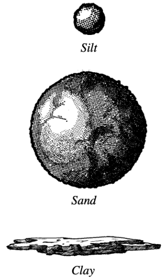
Figure 2. Soil particle sizes. The larger sand particles allow water to drain quickly through soil. Clay particles tend to pack more closely together, causing water to drain more slowly.
