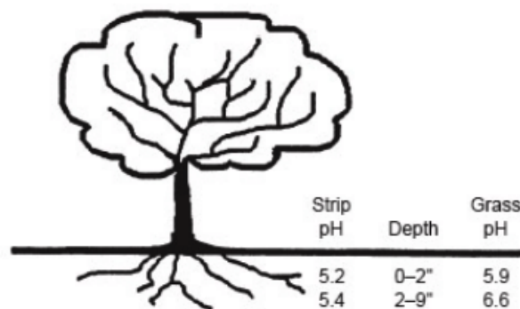
Figure 5. Soil pH differences from samples taken between rows and under the drip line. The figure also shows differences in soil pH with depth.
