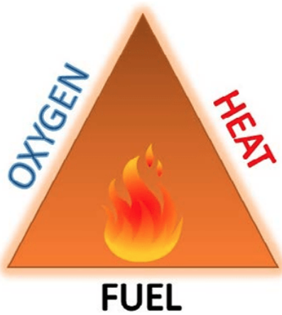
Figure 2. Fire triangle.
