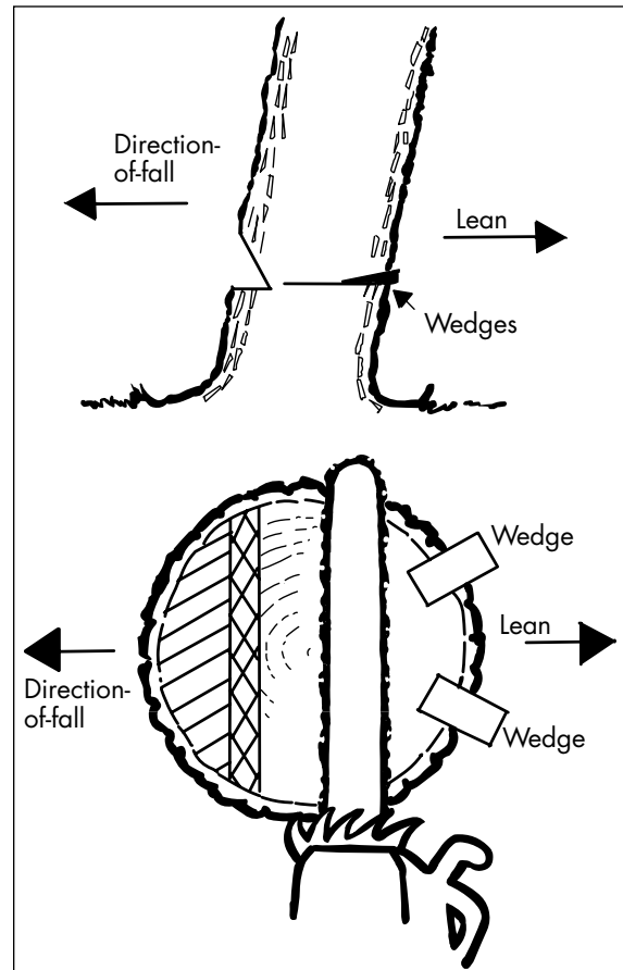
Figure 19.—Felling against the lean, using wedges.
