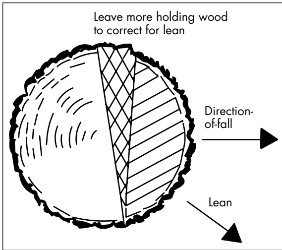
Figure 18.—Use “holding wood” to correct for moderate lean.
