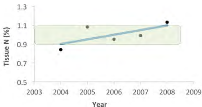
Figure 13.—Cranberry tissue N concentration from the same bed for 5 years. Figure by John Hart.
