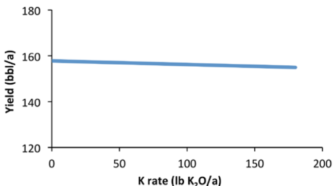
Figure 45.—Cranberry yield was not influenced by K application after 3 years of K treatments, 1998. Yield from both sites was similar, so a single line is used to represent both beds. Figure by John Hart.
