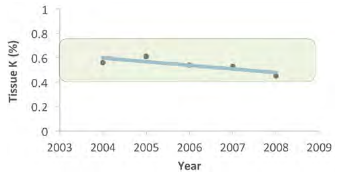
Figure 12—Cranberry tissue K concentration from the same bed for 5 years. The light green highlighted area is the K sufficiency range. Figure by John Hart.
