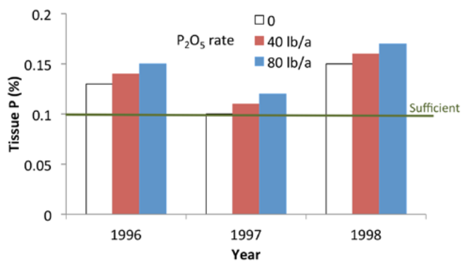
Figure 37.—Cranberry tissue P increased with P fertilizer application at the Coos County site. Figure by John Hart.
