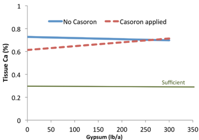
Figure 52.—Cranberry leaf Ca concentration increased with gypsum application only when Casoron was applied. All leaf Ca concentration values are within the sufficient range for cranberry. Unpublished data from Linda White; figure by John Hart.
