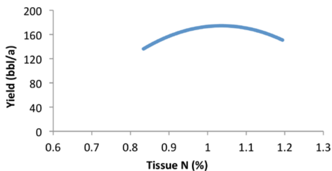
Figure 15.—Cranberry yield from an Oregon bed decreased as tissue N increased from 1 to 1.2 percent. Figure by John Hart.
