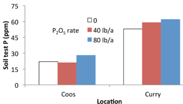
Figure 36.—Soil test P change with P fertilizer application (6-inch sample collection depth) in two south coastal Oregon cranberry beds. Figure by John Hart.
