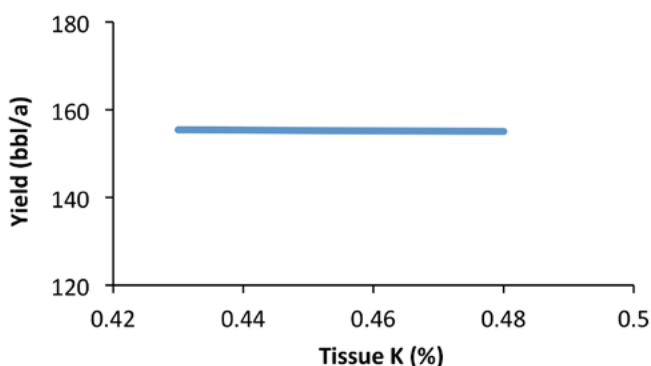
Figure 47.—Cranberry yield and leaf K concentration, 1998. Data from both sites are combined. Figure by John Hart.
