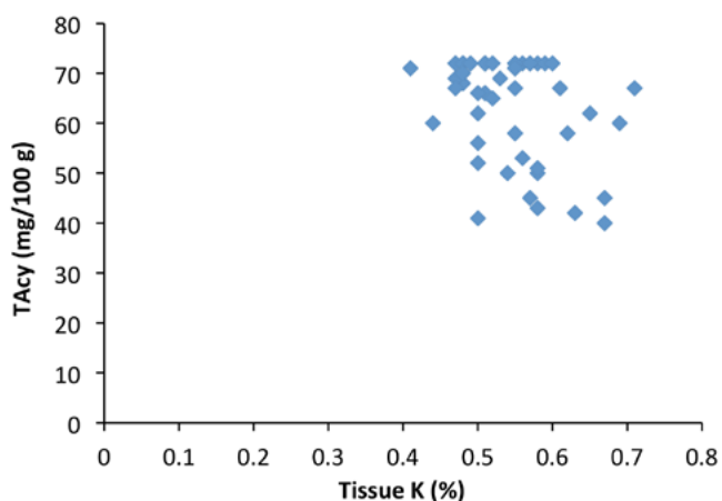
Figure 48.—TAc and leaf K concentration for the Curry County site, 1998. Figure by John Hart.
