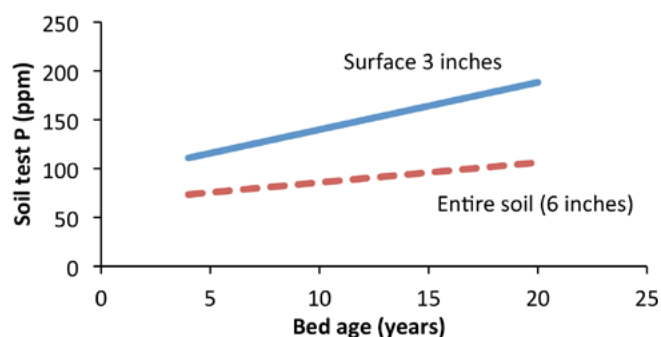
Figure 34.—Soil test P increased in the top 3 inches of soil with increasing cranberry bed age. Figure by John Hart.
