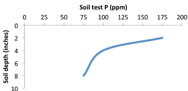
Figure 35.—Soil test P decreased with sampling depth in a 10-year-old cranberry bed. Figure by John Hart.
