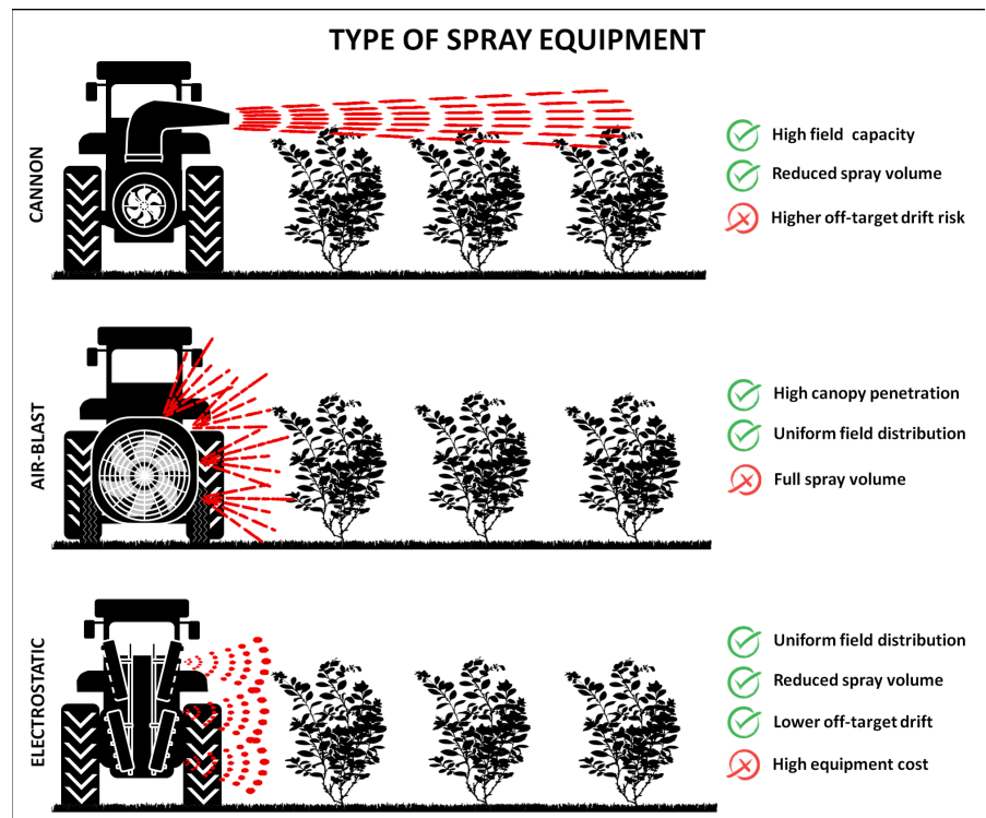
Figure 1. Advantages and disadvantages of three types of spray equipment used in small fruit production.
