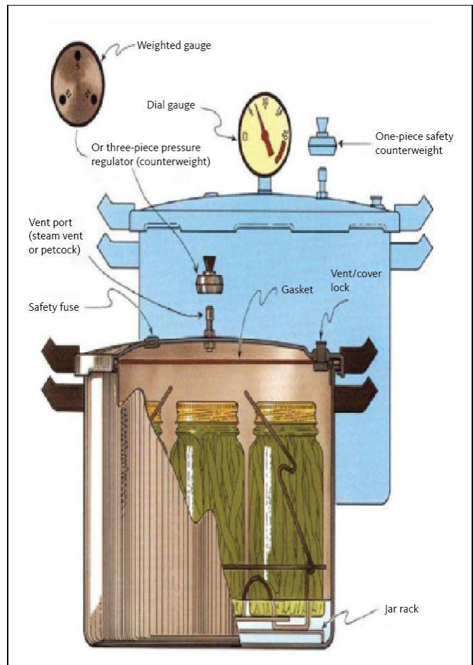
Pressure canner.
